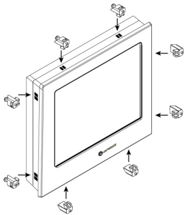
USP-104-B10: 8 mounting brackets
