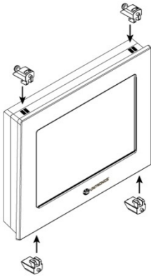
USP-070-B10: 4 mounting brackets
